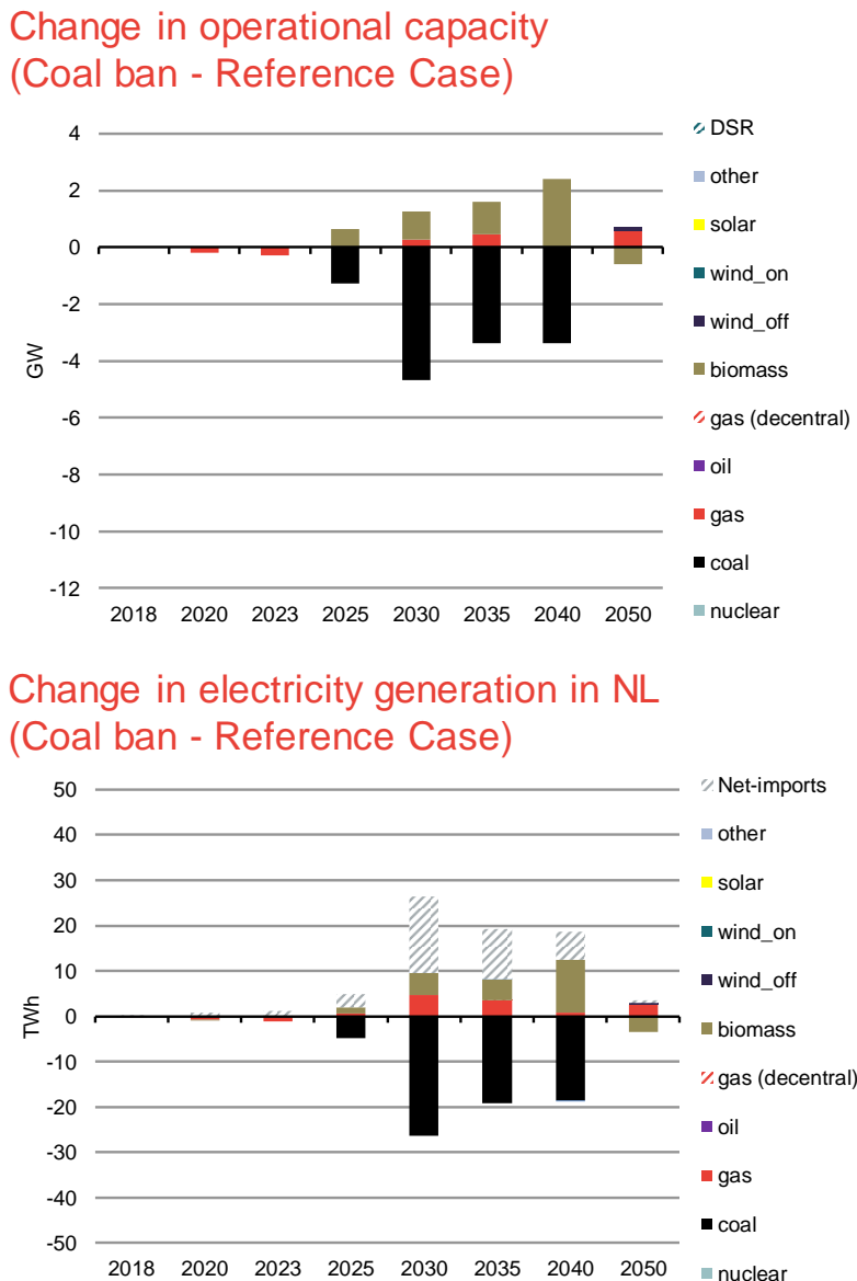
Figure 11 Coal ban - Impact on operation capacity and electricity supply in the Netherlands
